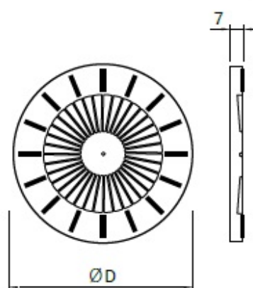
AWR-3-1-P0
