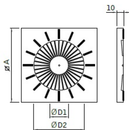
AWR-3-1-PK
